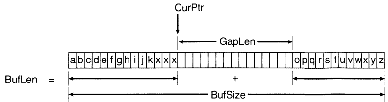
Figure 15.5 Buffer after undo
