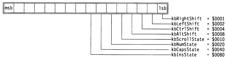
Figure 19.7 Keyboard state mask flags
