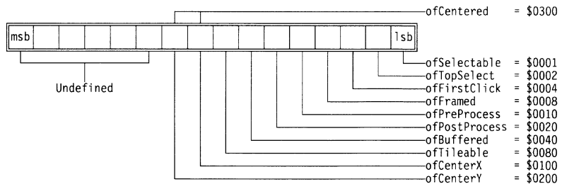
Figure 19.14 Options bit flags
