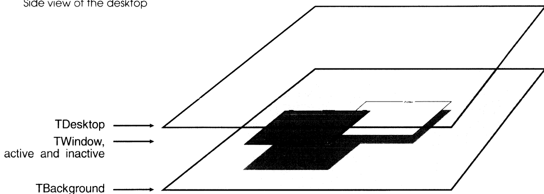
Figure 8.8 Side view of the desktop
