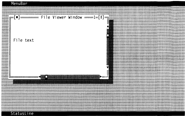
Figure 8.3 Desktop with file viewer added
