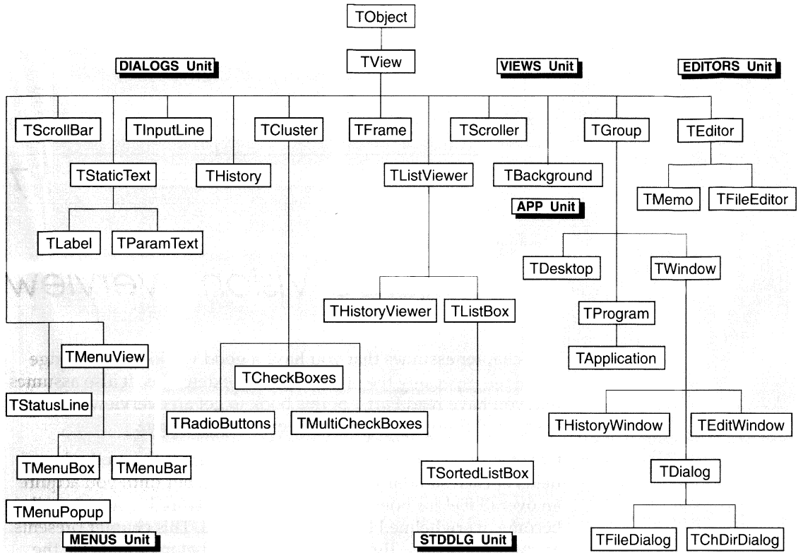
Figure 7.1: Turbo Vision object hierarchy
