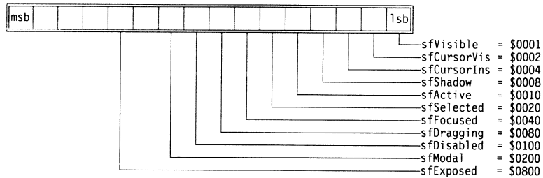
Figure 19.11 State flag bit mapping
