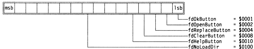
Figure 19.5 File dialog box option flags
