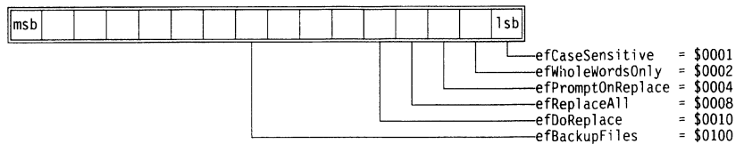
Figure 15.6 Editor flag bit mapping
