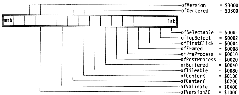
Figure 19.9 Options bit flags
