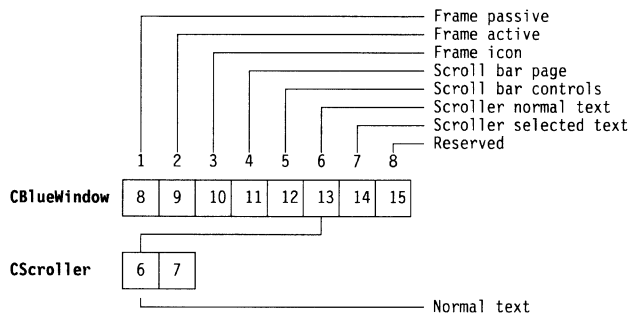
Figure 14.3 Mapping a scroller's palette onto a window
